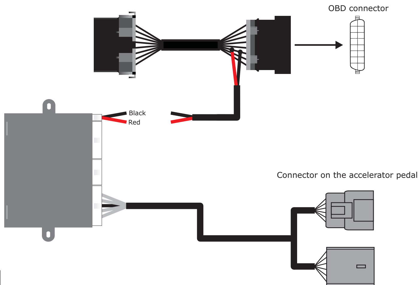
Dismount the originale OBD connector from the bracket, and connect the enclosed Y cable. Mount the other end of the Y cable in the bracket.
