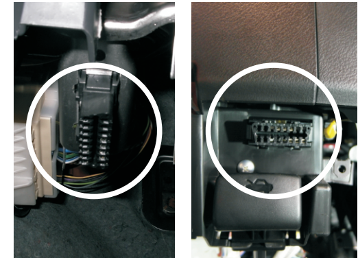
Dismount the originale OBD connecotor from the bracket, and connect the enclosed Y cable. Mount the other end of the Y cable in the bracket.
