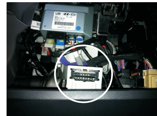
Dismount the originale OBD connecotor from the bracket, and connect the enclosed Y cable. Mount the other end of the Y cable in the bracket.
