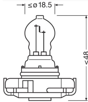
PS24W
