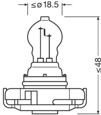
PS19W
