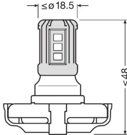
≙ PS19W
