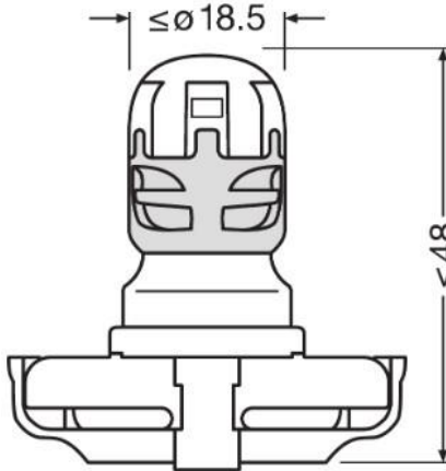
≙ PS19W
