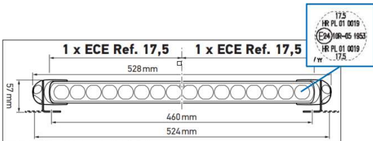
Joonis 1 - Hella Led Light Bar 470 Single Twin
